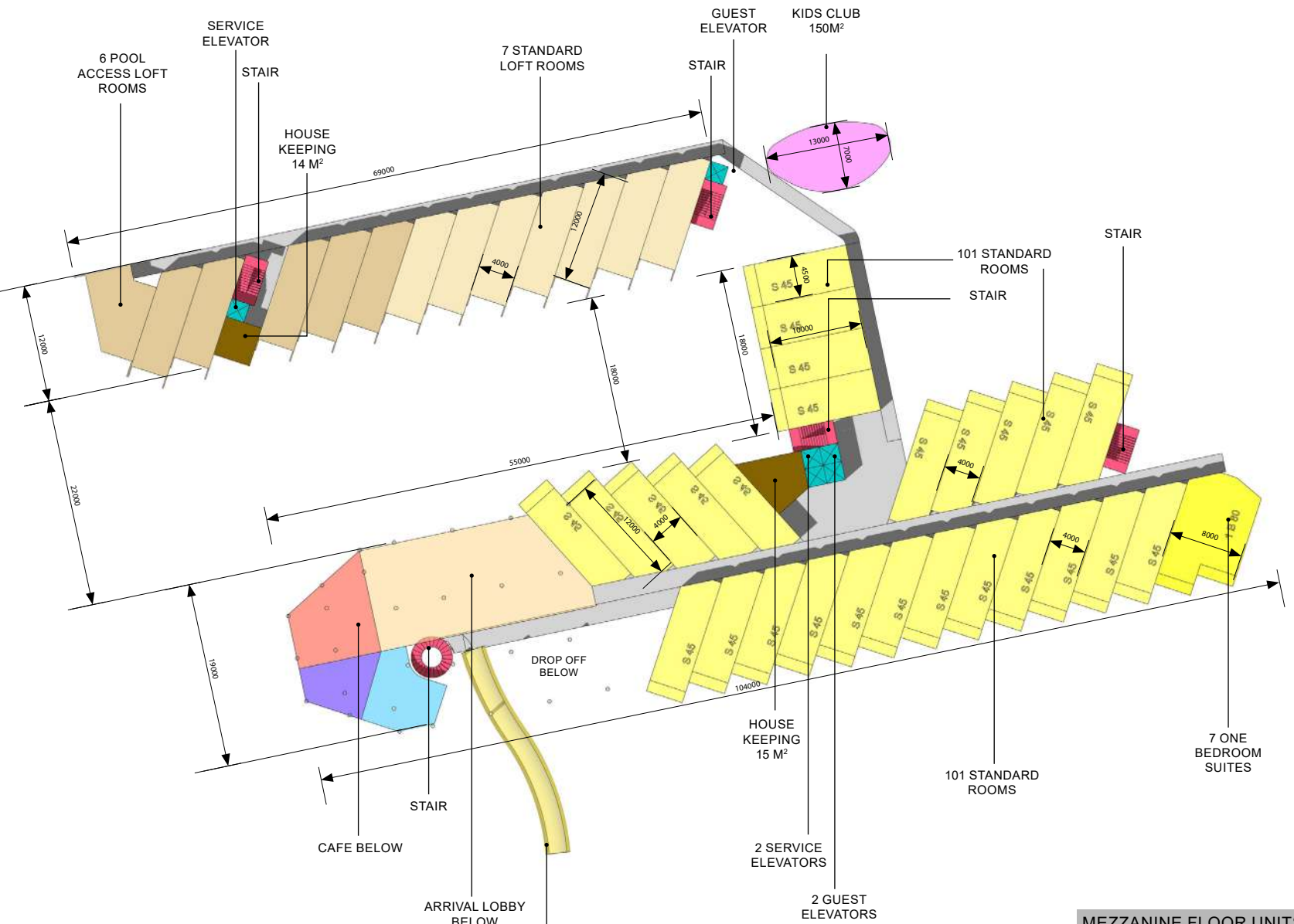
MEZZANINE FLOOR
