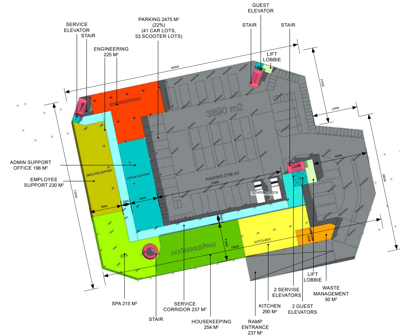
BASEMENT FLOOR
